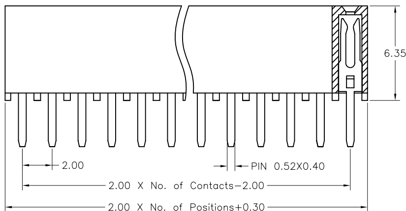
FBS2631 Series FBS1631 Series
