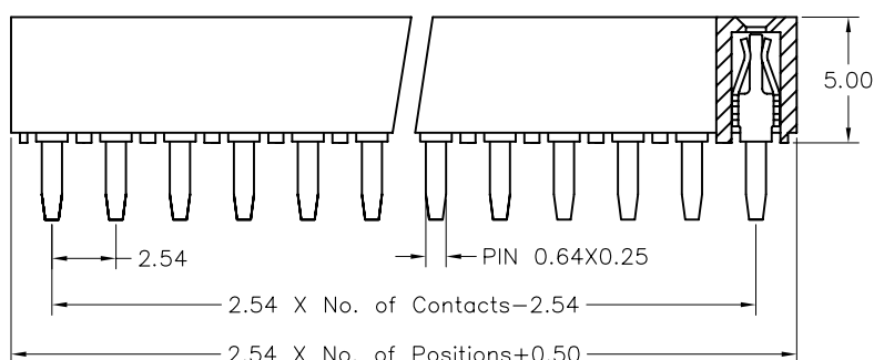
FAF1501 Series
