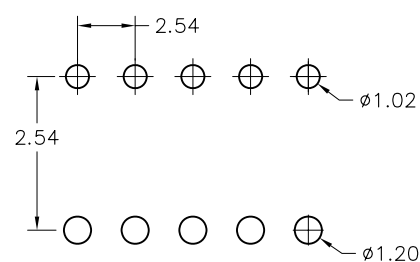
FAF2501 Series
