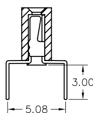
FAF1501 Series
