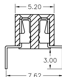
FAF2501 Series
